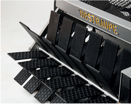
Gentle fruit collection with plastic fins
